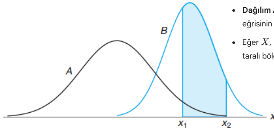
Figure : P(x_1 < X < x_2) for different normal curves.
